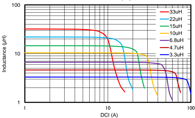
Characteristics of DC Superposition
