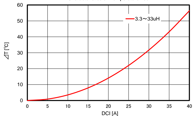
Characteristics of Temperature rise
