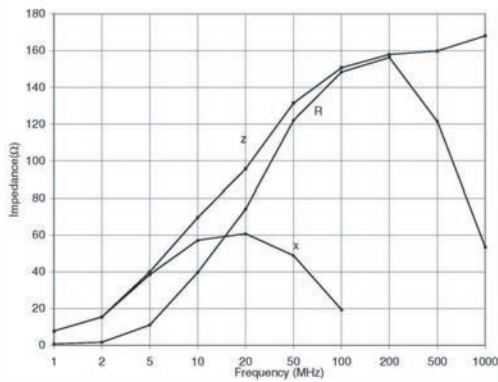
Z-f Characteristics
